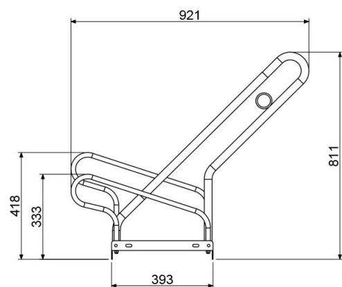
S01+ L01 BIKE RACK DIMENSIONS
