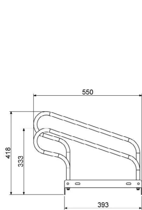
S01 BIKE RACK DIMENSIONS
