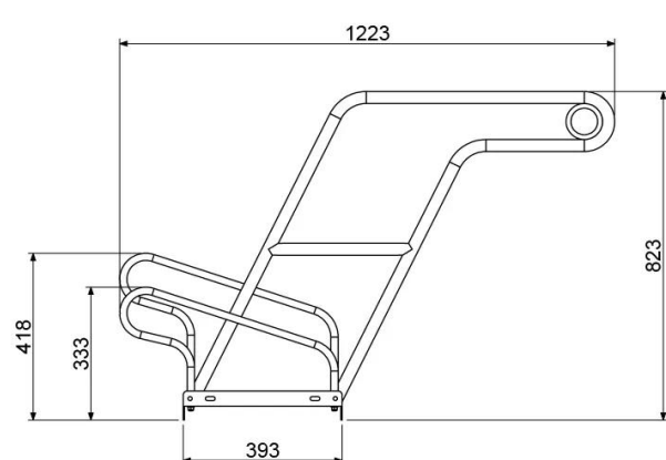
S01+ L02 BIKE RACK DIMENSIONS
