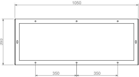
1050 MM BASE DIMENSIONS
