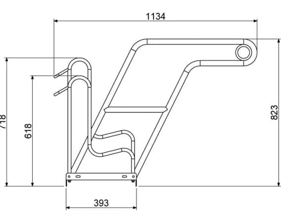
S02+ L02 FLOOR BIKE RACK DIMENSIONS
