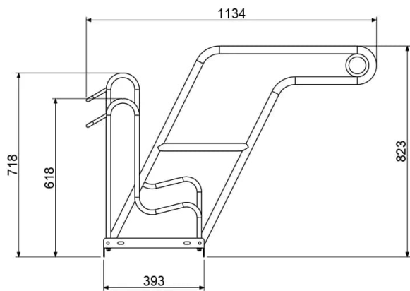
S02+ L02 FLOOR BIKE RACK DIMENSIONS
