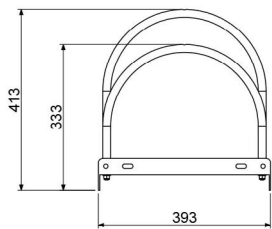
S03 BIKE RACK DIMENSIONS
