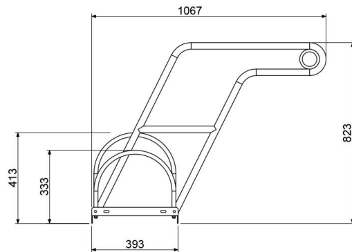
S03+ L02 BIKE RACK DIMENSIONS
